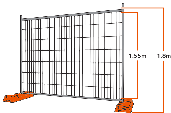
FIGURE 1 Standard Temporary Fence Measurements
